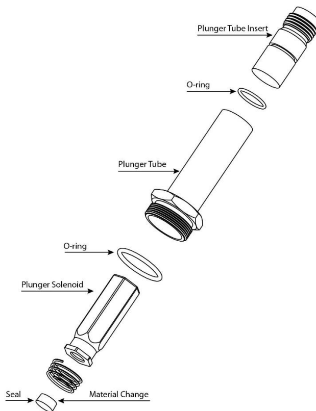
Figure 1 - Plunger Assembly Seal Location
