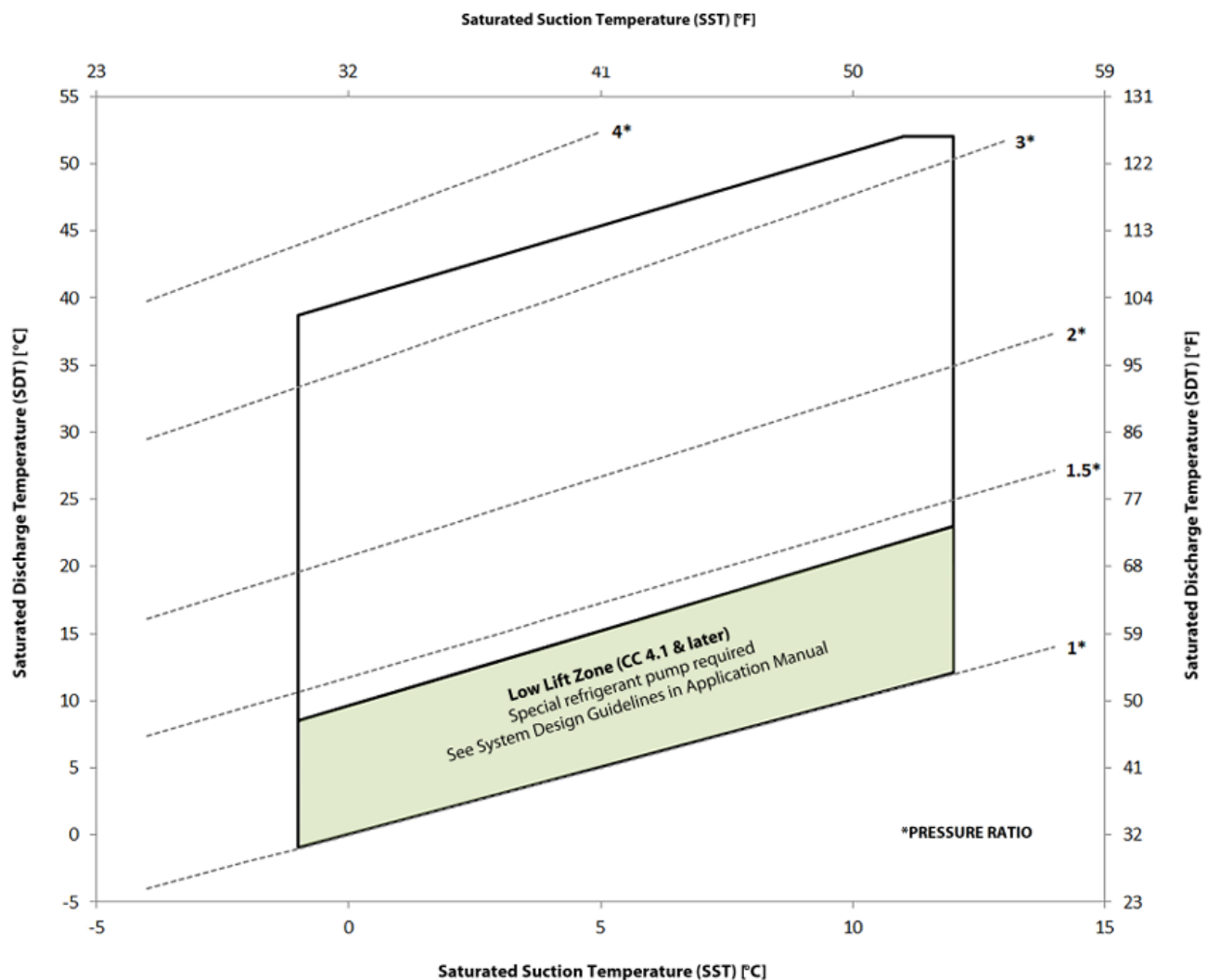
Figure 1 – Operating Envelope, High SST: TTS650
