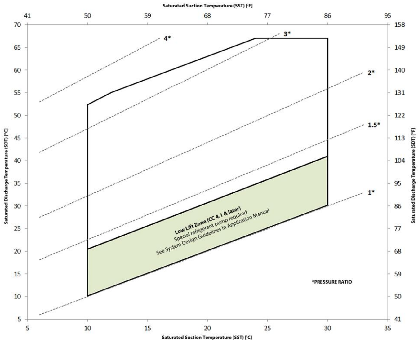
Figure 2 – Operating Envelope, High SST: TGS510
