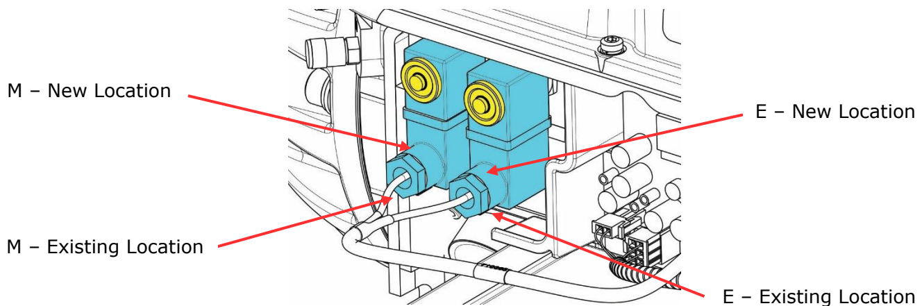
Figure 1 – Motor and Electronics Cooling Marking Locations
