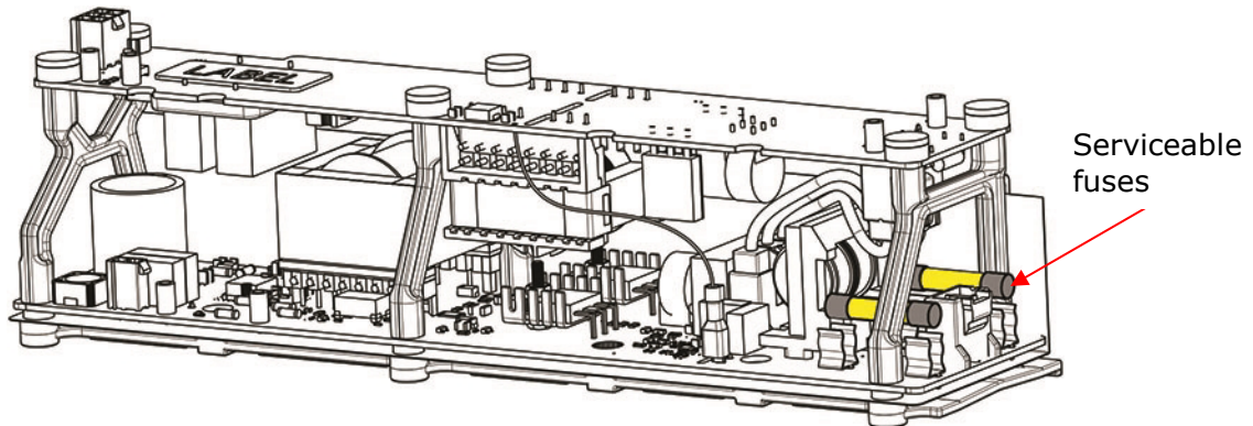
Figure 1 – DC-DC Converter Fuses
