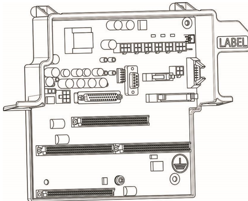
Figure 1 –New Style Backplane (Kit 100021-2)
