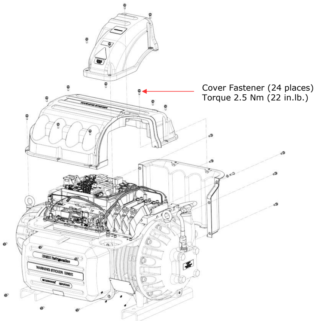
Figure 1 – Cover Screw Torque
