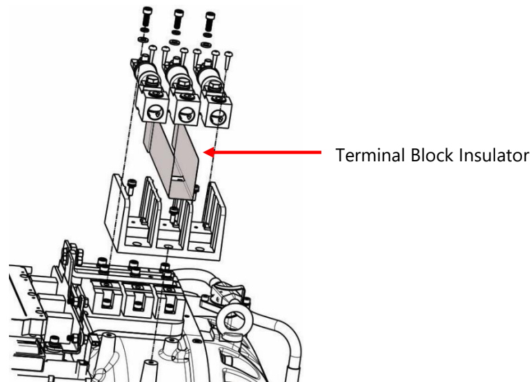
Figure 1 – Terminal Block Isolator
